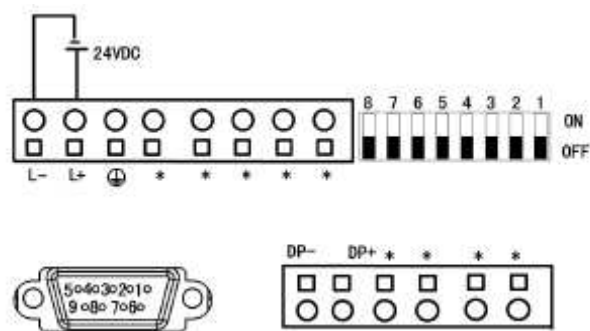
Figure 3-3-2 LM3401 Terminal Definition & Wiring
