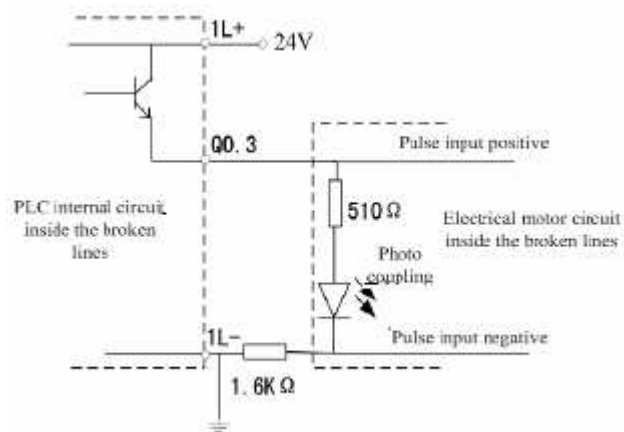
Figure 2-7-3 LM3108 High-Speed Output & Motor Wiring Example 2 (Q1.1 same wiring)
