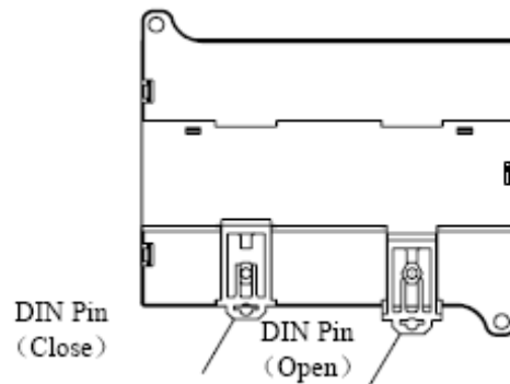
Figure 4-3-5 Rail Pin
