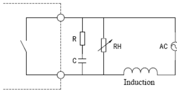
Figure 4-2-4 AC Relay Protection
