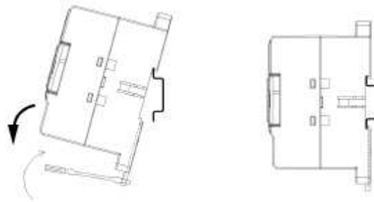
Figure 4-3-6 Rail Installation
