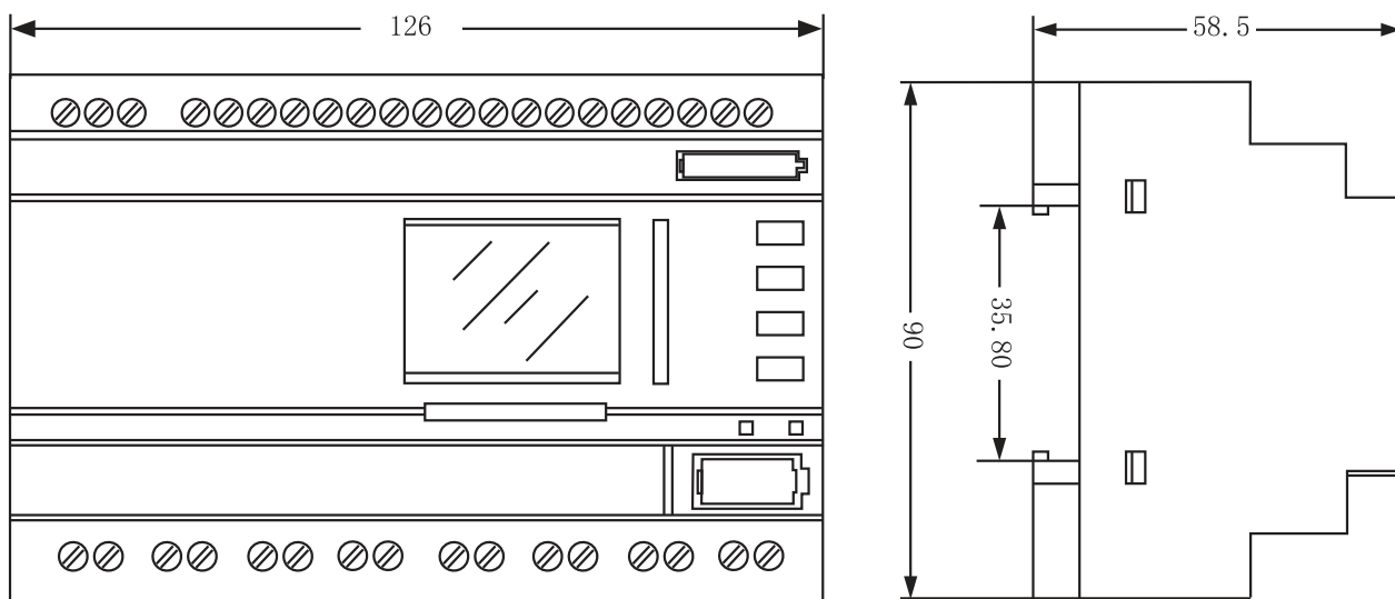
Installation Dimension of APB- 22 Series (mm)
