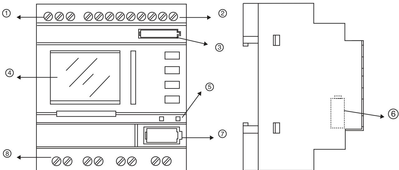
Fig. 1.1 APB- 12 Series Main Machine
