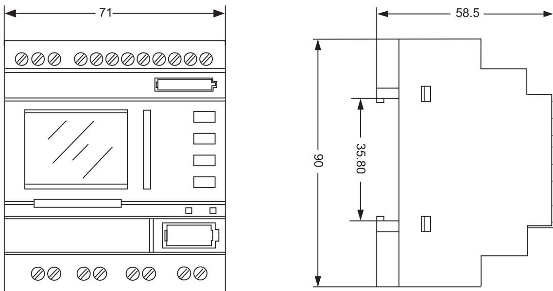
Installation Dimension of APB- 12 Series (mm)
