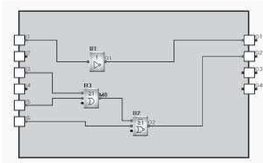
Fig 4 . 15 Link the line between blocks
