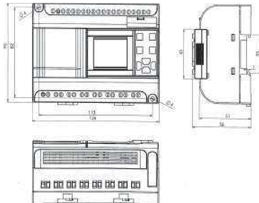
Fig 2.3 AF-20 FAB Series installation dimensions (Unit: mm)
