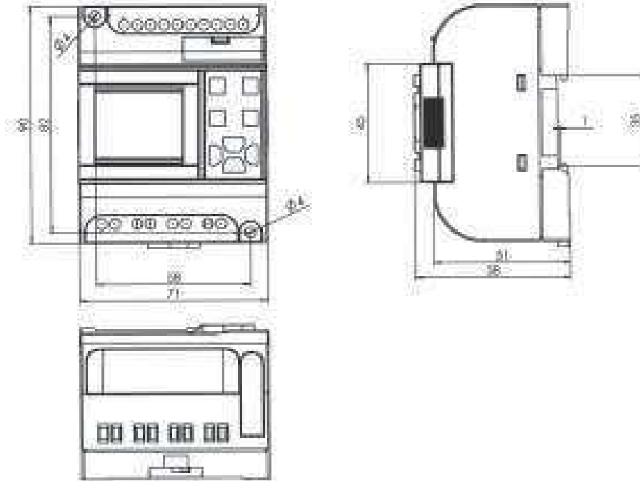
Fig 2.3 AF-10 FAB Series installation dimensions (Unit: mm)
