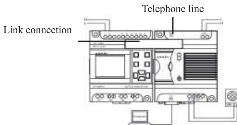
Fig 6.2 Connection Between FAB and AF-MUL
