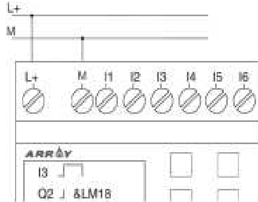
Fig 2.8 DC Type ( E Type)
